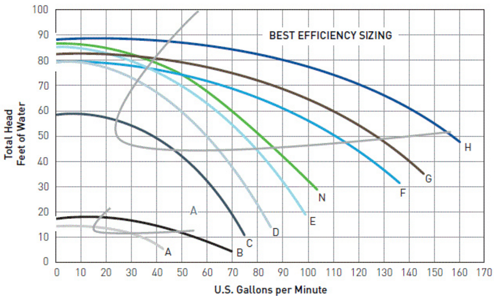
60 Hz Performance Curve
