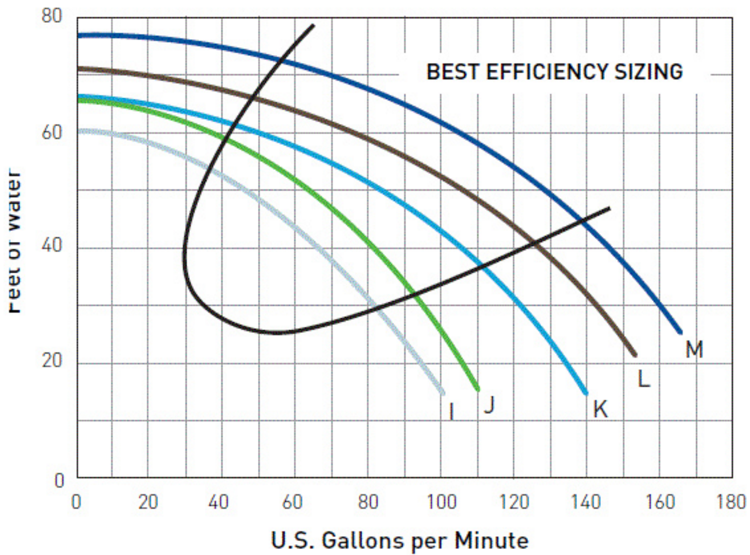
50 Hz Performance Curve
