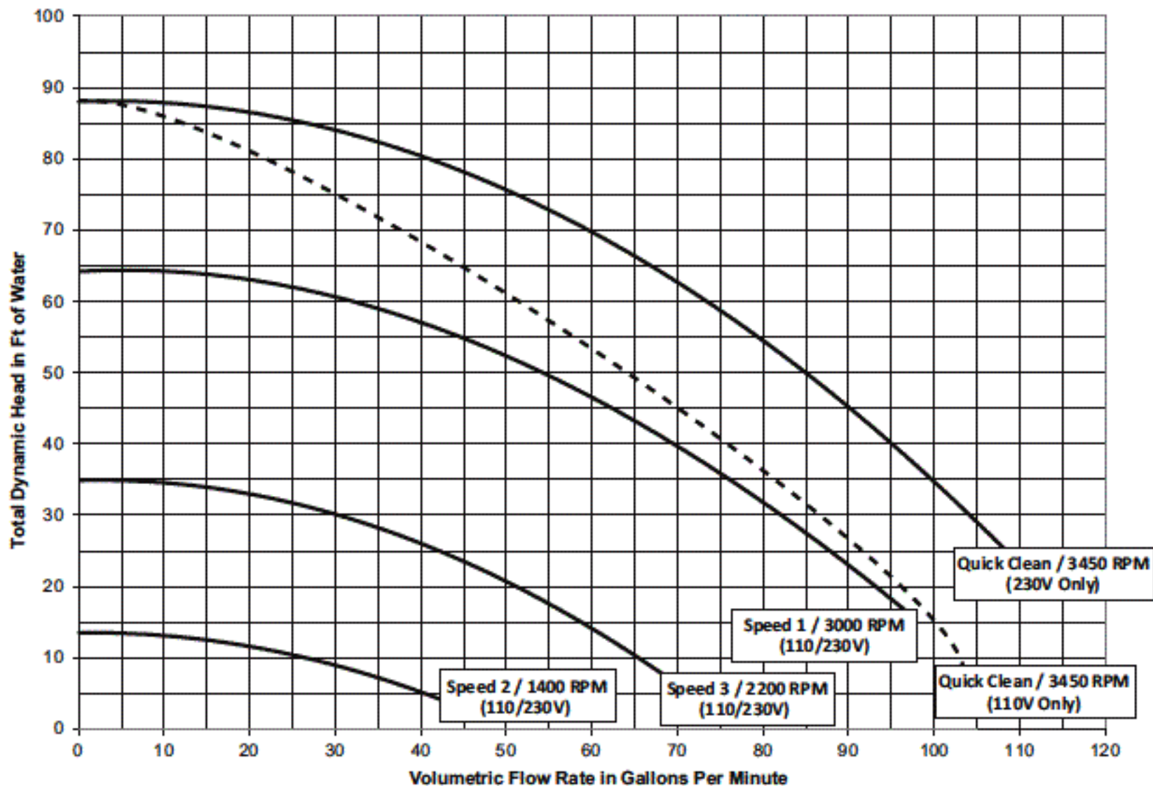
SuperFlo® VS Performance Curves for Preset Speeds
